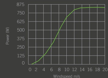
Power curve
